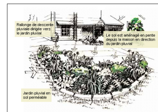
Figure 1. Jardin pluvial
